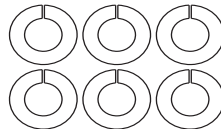
Z06 Ø10.2xØ18.4x2.5T
