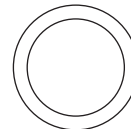
Z23 Ø26.4xØ33.9x0.3T
