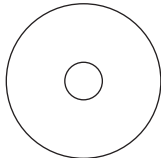
Z02 Ø10.5xØ42x1.5T
