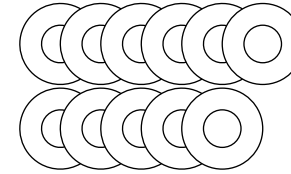
Z09 Ø10.2xØ22x2.0T
