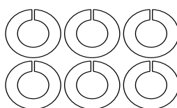
Z02 12.2xØ21.5x3.0T
