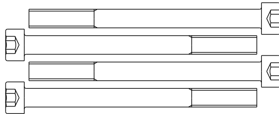
Z05 M10x125L-35L
