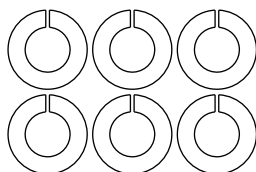
Z02 12.2xØ21.5x3.0T
