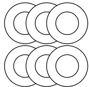
Z01 Ø12.2xØ22x2.0T
