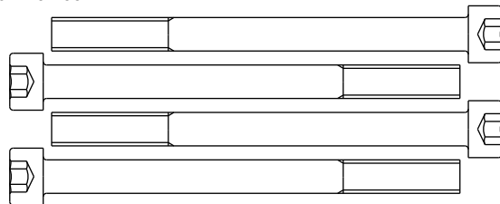
Z05 M10x125L-35L
