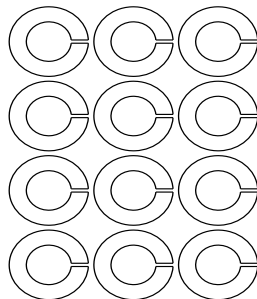
Z02 Ø12.2xØ21.5x3.0T
