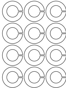
Z02 Ø12.2xØ21.5x3.0T
