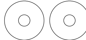
Z11 Ø10.2xØ35x2.0T
