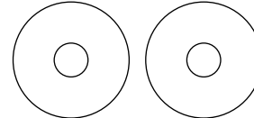
Z11 Ø10.2xØ35x2.0T
