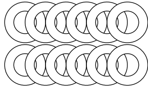
Z01 Ø12.2xØ22x2.0T
