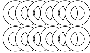
Z01 Ø12.2xØ22x2.0T
