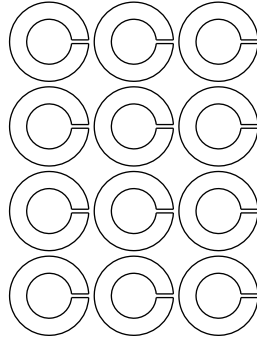
Z02 Ø12.2xØ21.5x3.0T
