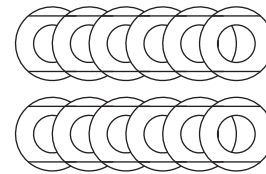
Z08 (ARC WASHER) Ø10.2xØ20.0x1.5T
