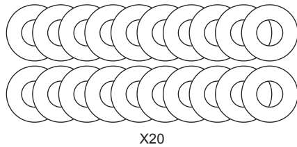
Z03 Ø10.2xØ 22.0x2.0T
