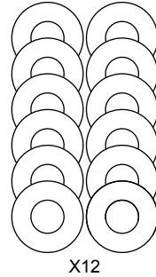
Z09 Ø10.2xØ22.2x2.0T
