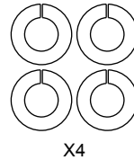
Z09 Ø10.2xØ22.2x2.0T
