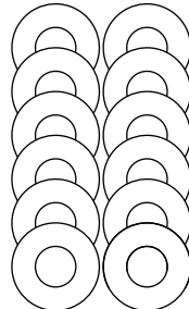
Z09 Ø10.2xØ22.2x2.0T
