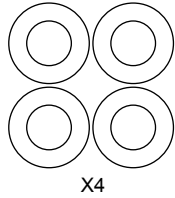
Z02 Ø12.2xØ21.5x3.0T
