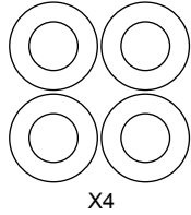
Z02 Ø12.2xØ21.5x3.0T
