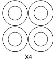
Z02 Ø12.2xØ21.5x3.0T
