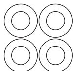
Z01 Ø12.2xØ22x2.0T
